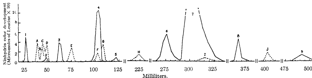
Fig. 1.—Analytical fractionation of streptolin AB hydrolysate on Dowex-50: —, streptolin hydrolysate; - - -, known amino acids: A, aspartic acid; B, serine; C, threonine; D, glutamic acid; E, glycine; F, ammonia; G, valine; H, \alpha,\gamma -diaminobutyric acid; I, lysine; J, arginine.
